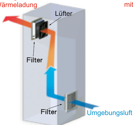
Abb.1 Abluftsystem
